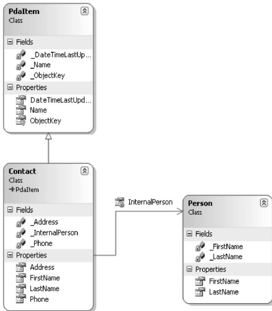
FIGURE 6.2: Simulating Multiple Inheritance Using Aggregation
