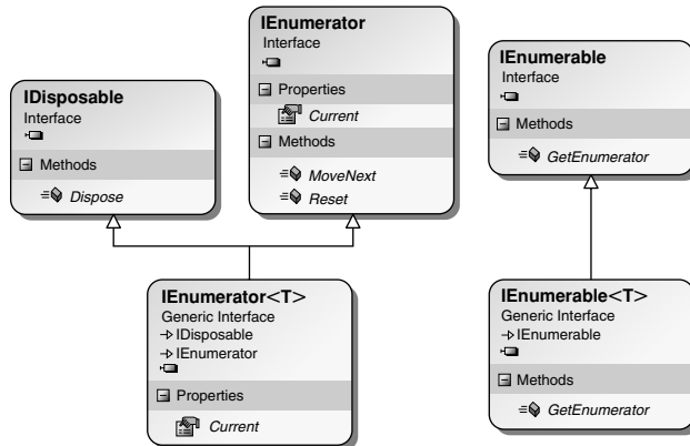
FIGURE 14.1: A Class Diagram of IEnumerator<T> and IEnumerator Interfaces
