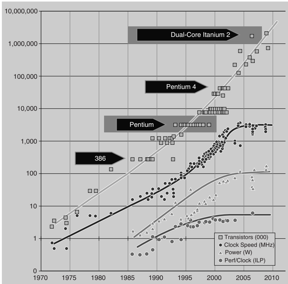
FIGURE 18.1: Clock Speeds over Time
