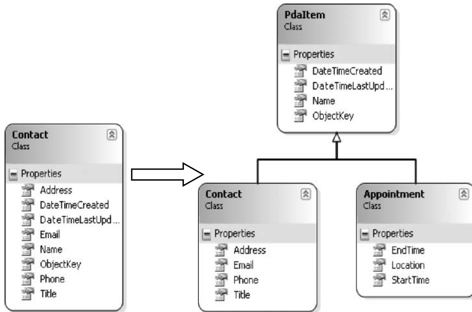
FIGURE 6.1: Refactoring into a Base Class
