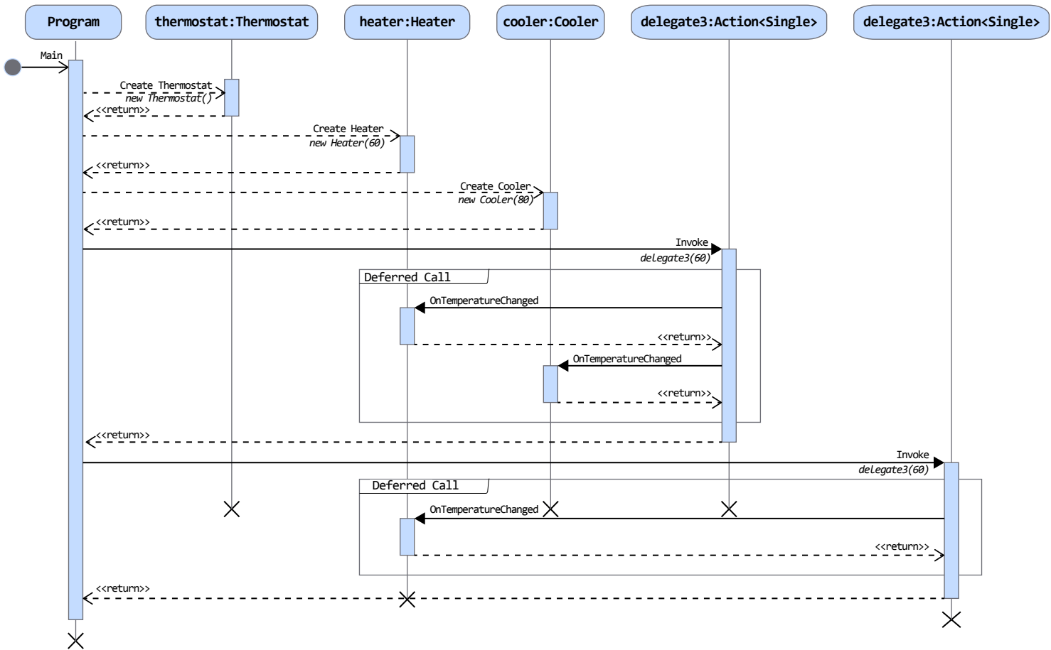
FIGURE 13.1: Delegate Invocation Sequence Diagram
