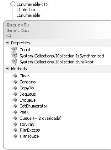
FIGURE 16.6: Queue<T> Class Diagram
