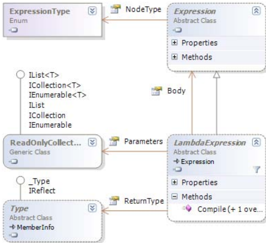
FIGURE 12.3: The Lambda Expression Tree Type
