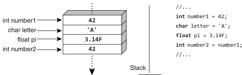
FIGURE 8.1: Value Types Contain the Data Directly
