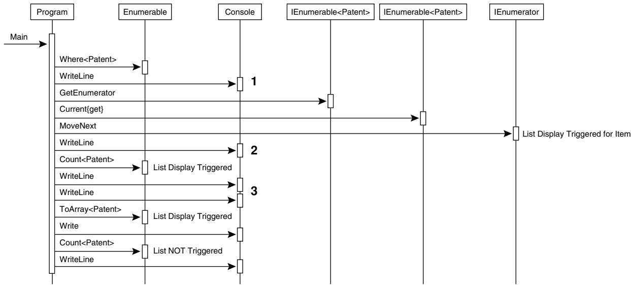
FIGURE 14.2: Sequence of Operations Invoking Lambda Expressions
