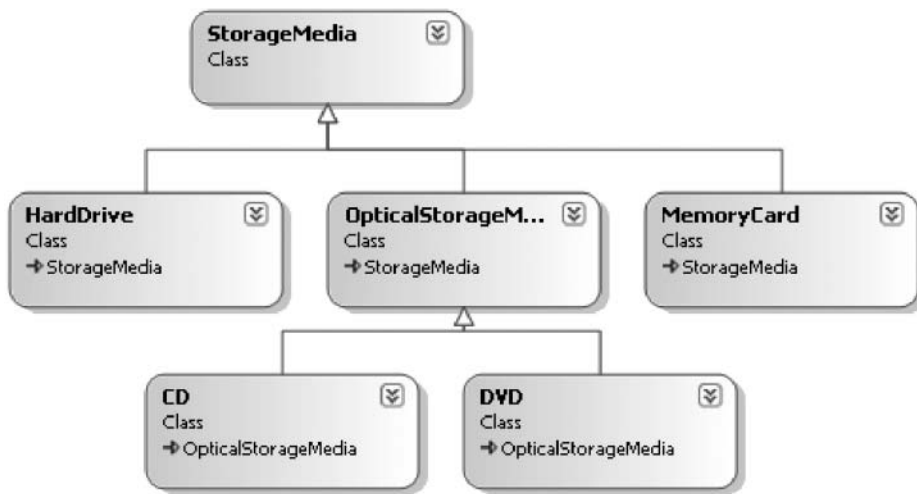
FIGURE 5.1: Class Hierarchy
