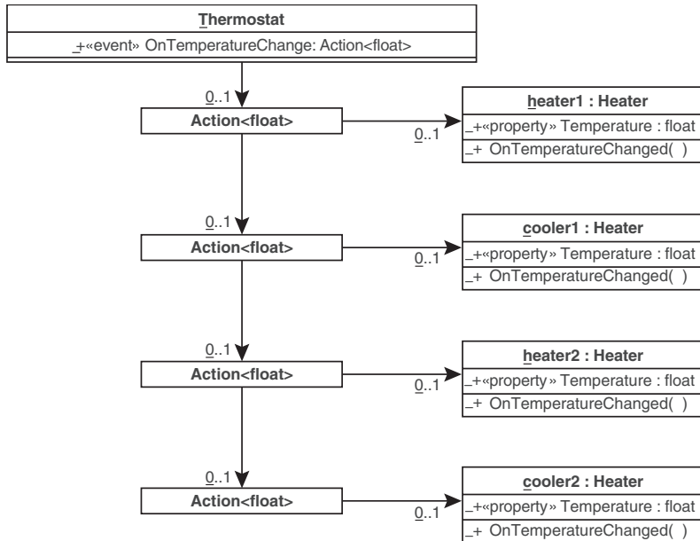
FIGURE 13.2: Multicast Delegates Chained Together
