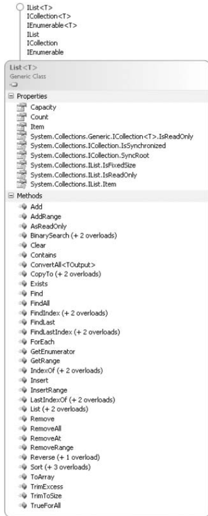
FIGURE 16.2: List<> Class Diagrams
