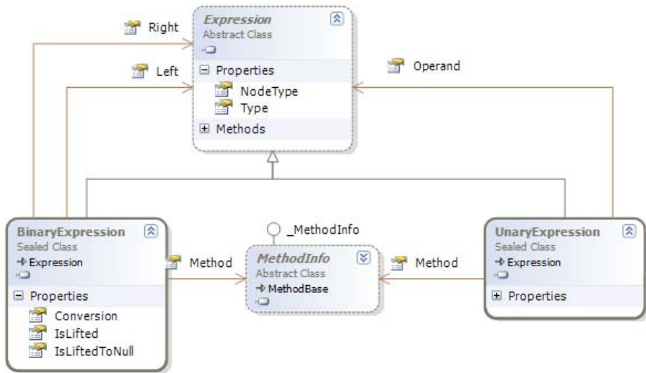
FIGURE 12.4: Unary and Binary Expression Tree Types
